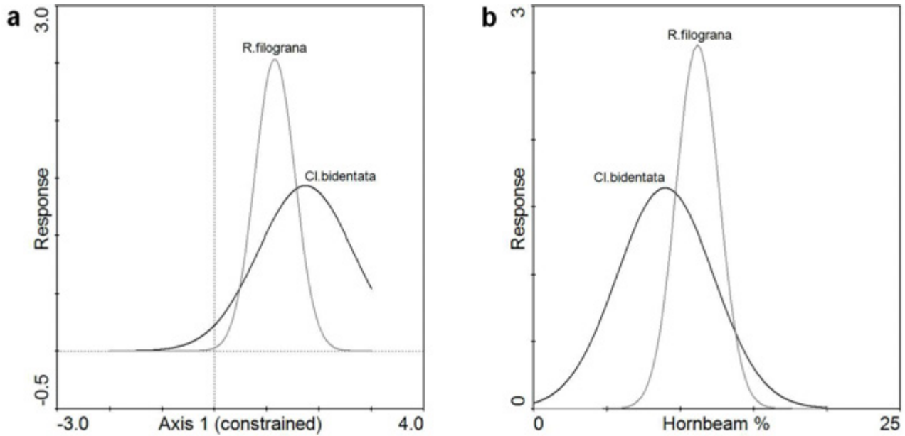
Figure 6 Response curves of R. filograna and C. bidentata describing relation between the species and: (a) the first ordination axis, interpreted as proportion of litter-covered against herb-covered area; and (b) the percentage of hornbeam leaves in the litter
