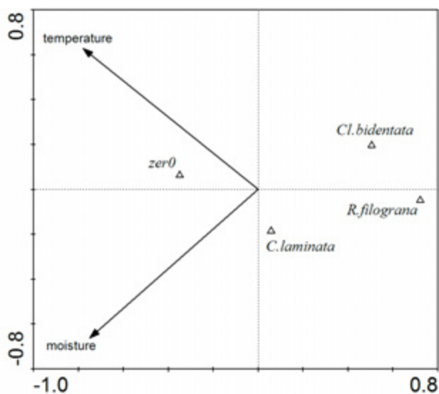
Figure 5 Ordination (CCA) diagram showing variation in the abundances of snail taxa (triangles) among different values of soil moisture and temperature (arrows); zer0 : samples with no Clausiliidae
