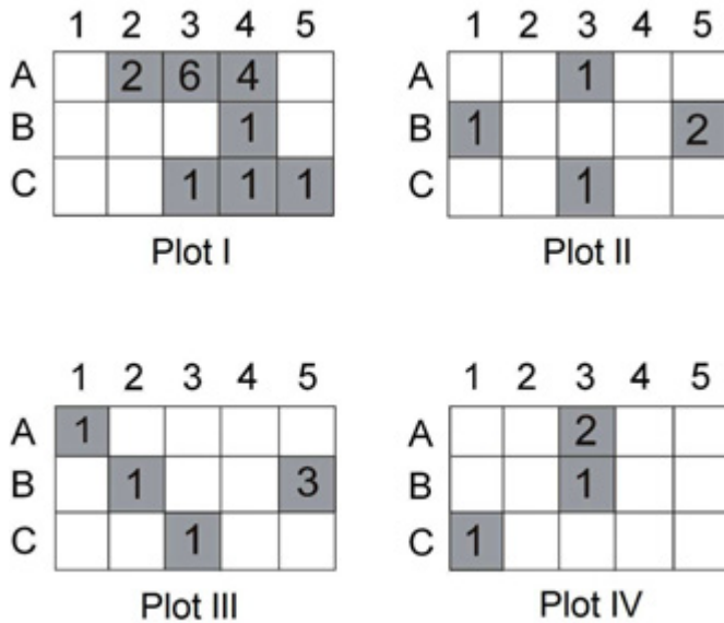
Figure 3 Spatial distribution and abundance of clausiliids in the sampling plots, 1–6 number of individuals: A - Ruthenica filigrana , B - Cl. bidentata , C - C. laminata
