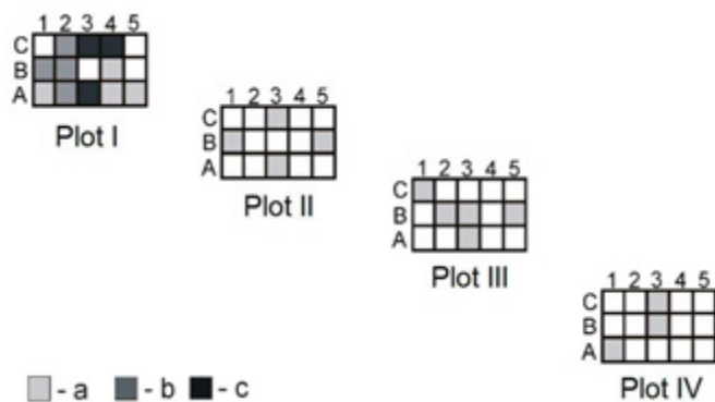
Figure 1 Spatial distribution and co-occurrence of clausiliids in the nature reserve Dębno in the sampling plots: a – one species, b – two species, c – three species
