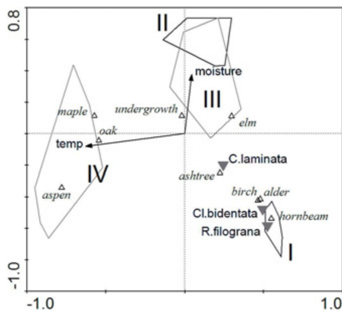
Figure 2 Correspondence Analysis triplot, showing composition of litter (hollow triangles) in the plots sampled (I-IV). The most outstanding samples from each area connected with solid lines. Snail species (solid inverted triangles) and soil temperature/moisture data (arrows) were included in the analysis as supplementary environment data (not influencing the ordination)
