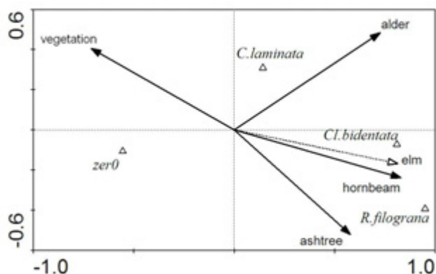
Figure 4 Ordination (CCA) diagram showing variation in the abundances of snail taxa (triangles) among different litter components (arrows); zer0 : samples with no Clausiliidae; dotted line: variable which was not significant according to Monte Carlo permutation test
